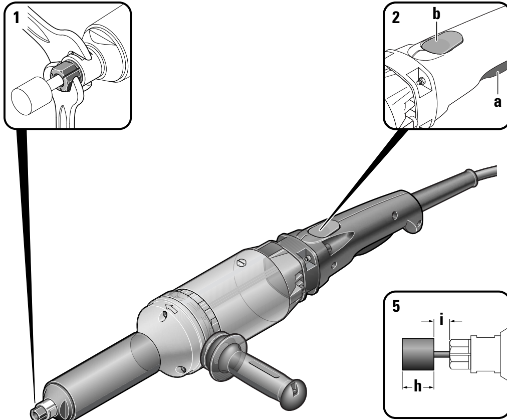
MSho852-12V
